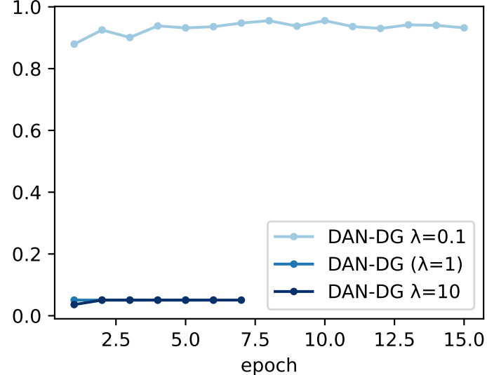
(f) study: mean source-val macro-F1
