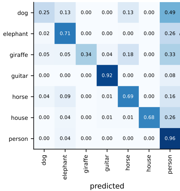
Source-only (acc 0.589)
