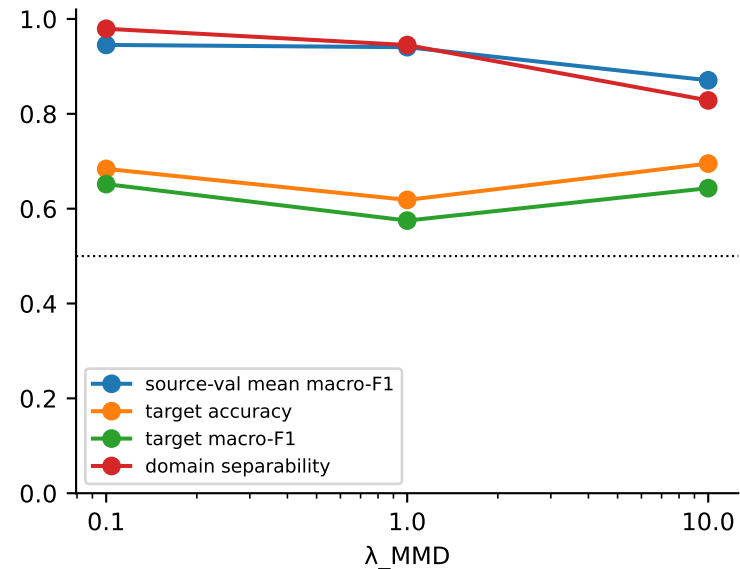
(a) alignment strength
