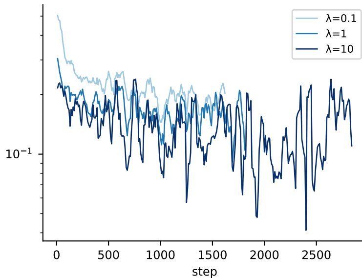
(b) MMD 2 during training
