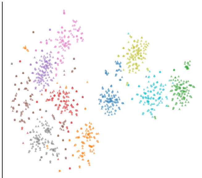
patch_shuffle
