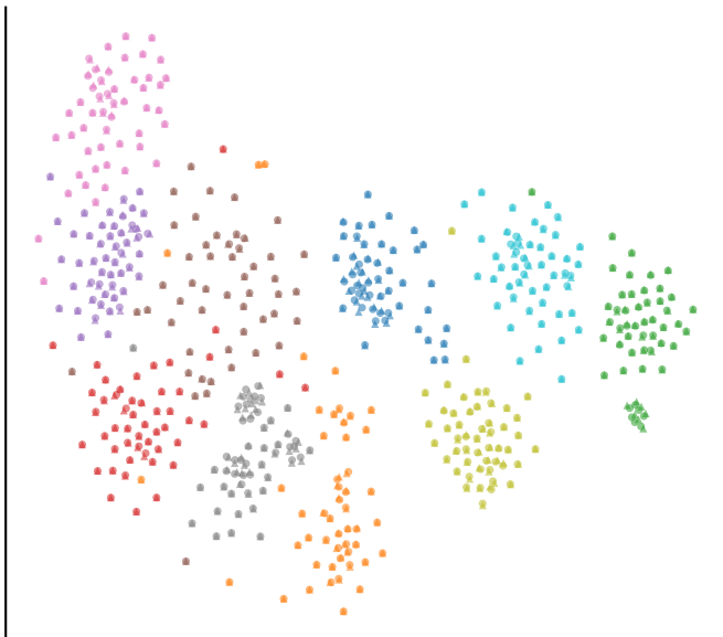
translation
