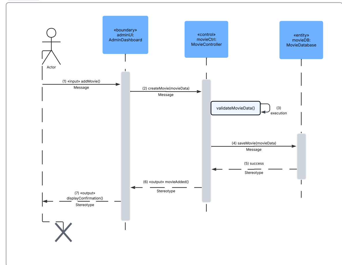
Sequence diagram
