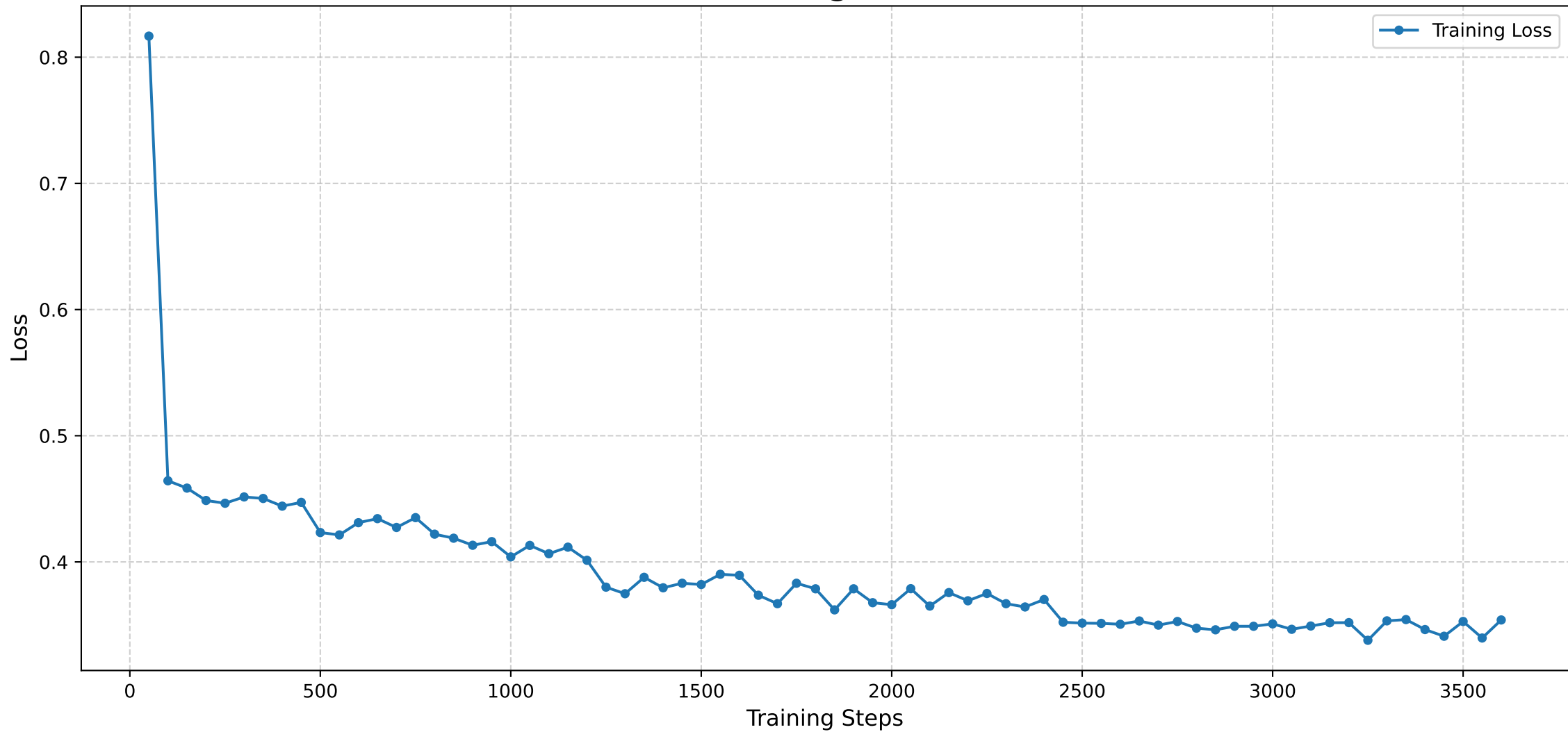
GPT-2 Training Loss Curve
