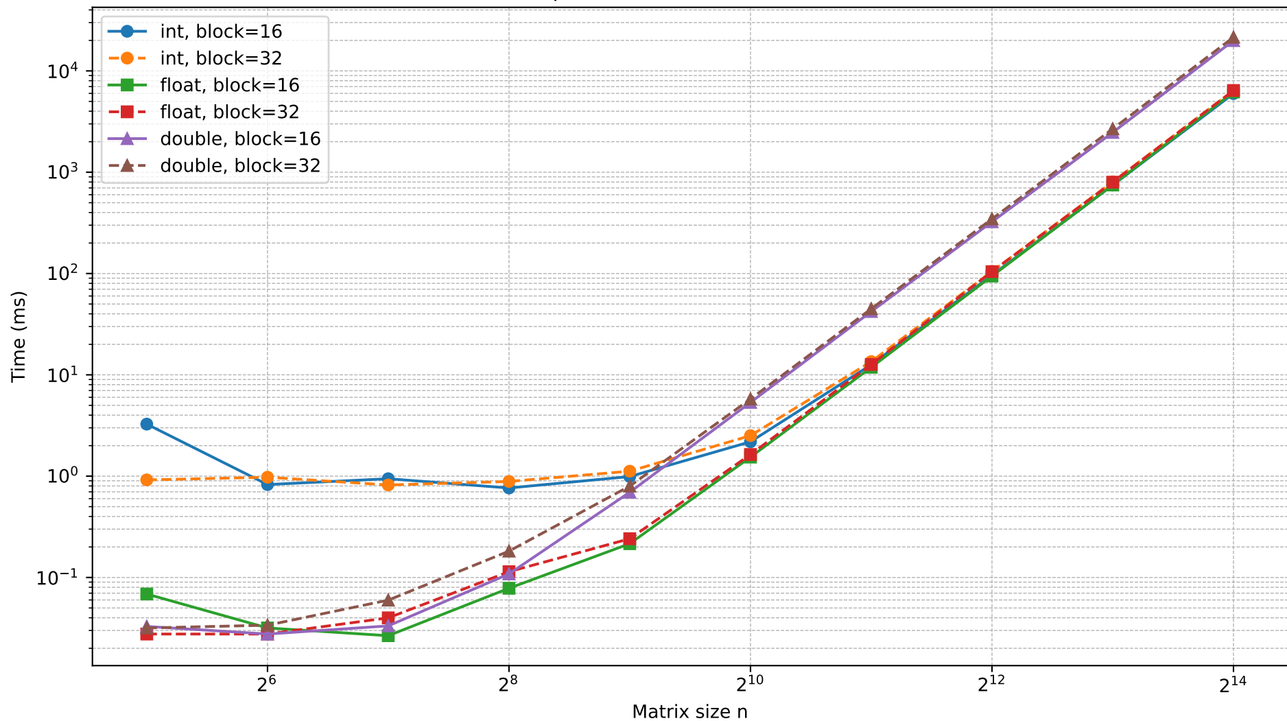
Tiled Matrix Multiplication Performance for int, float, double
