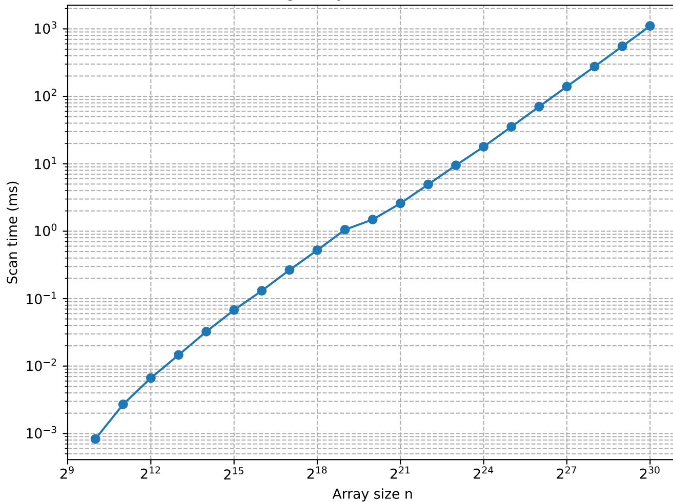
Scaling analysis of inclusive scan
