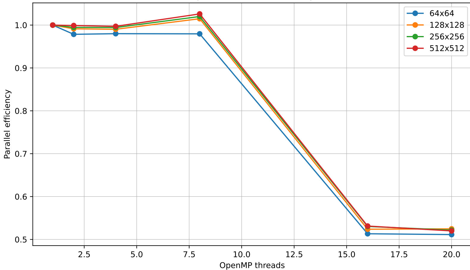
OpenMP Parallel Efficiency
