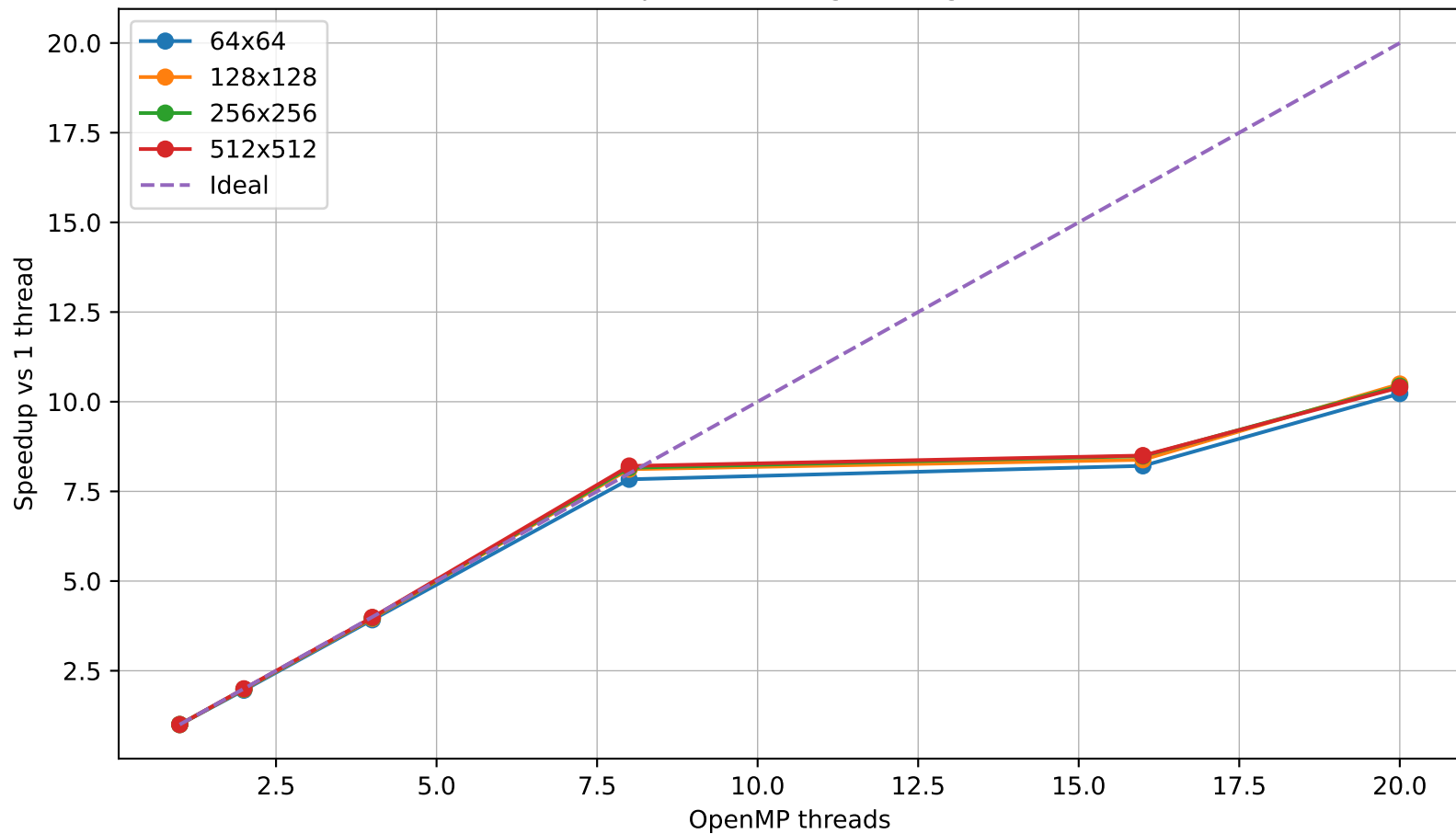
OpenMP Strong Scaling
