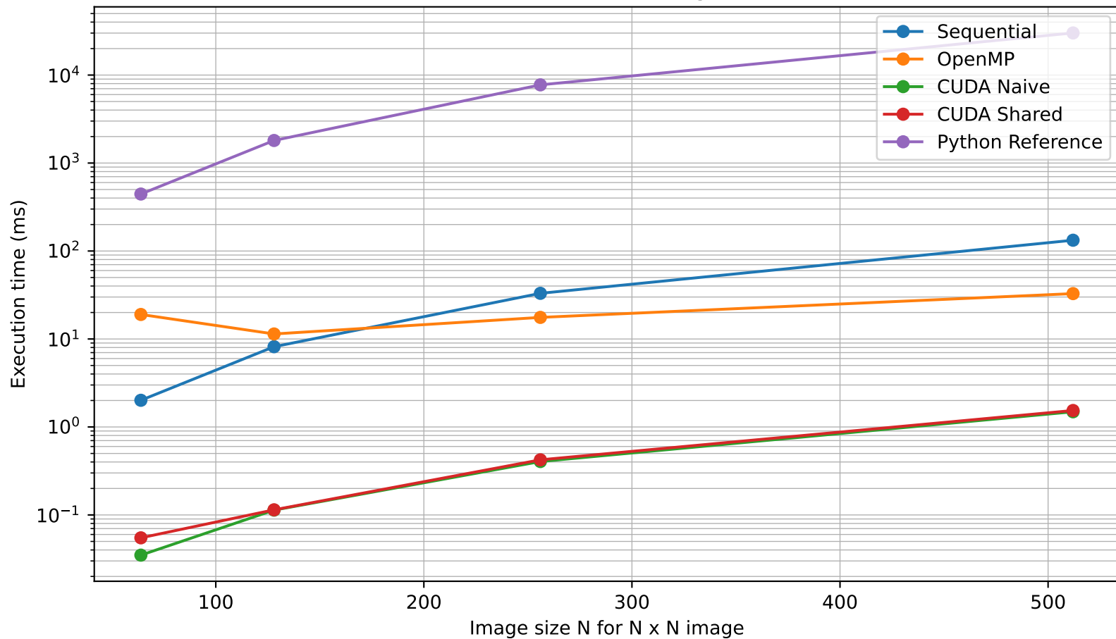
Execution Time vs Image Size
