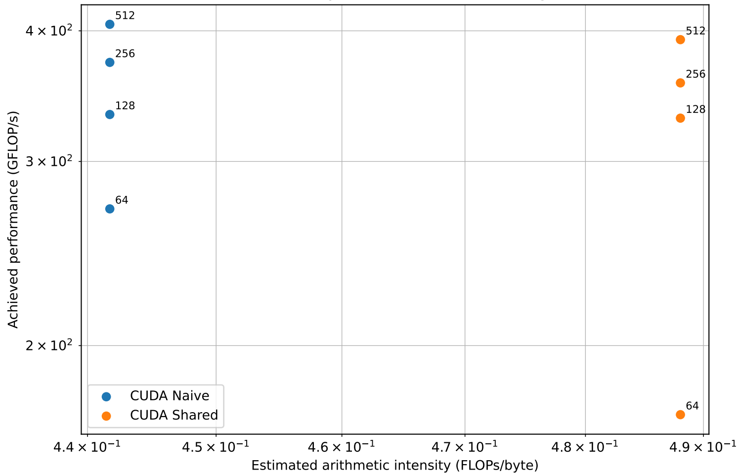
Roofline-Style CUDA Kernel Positioning
