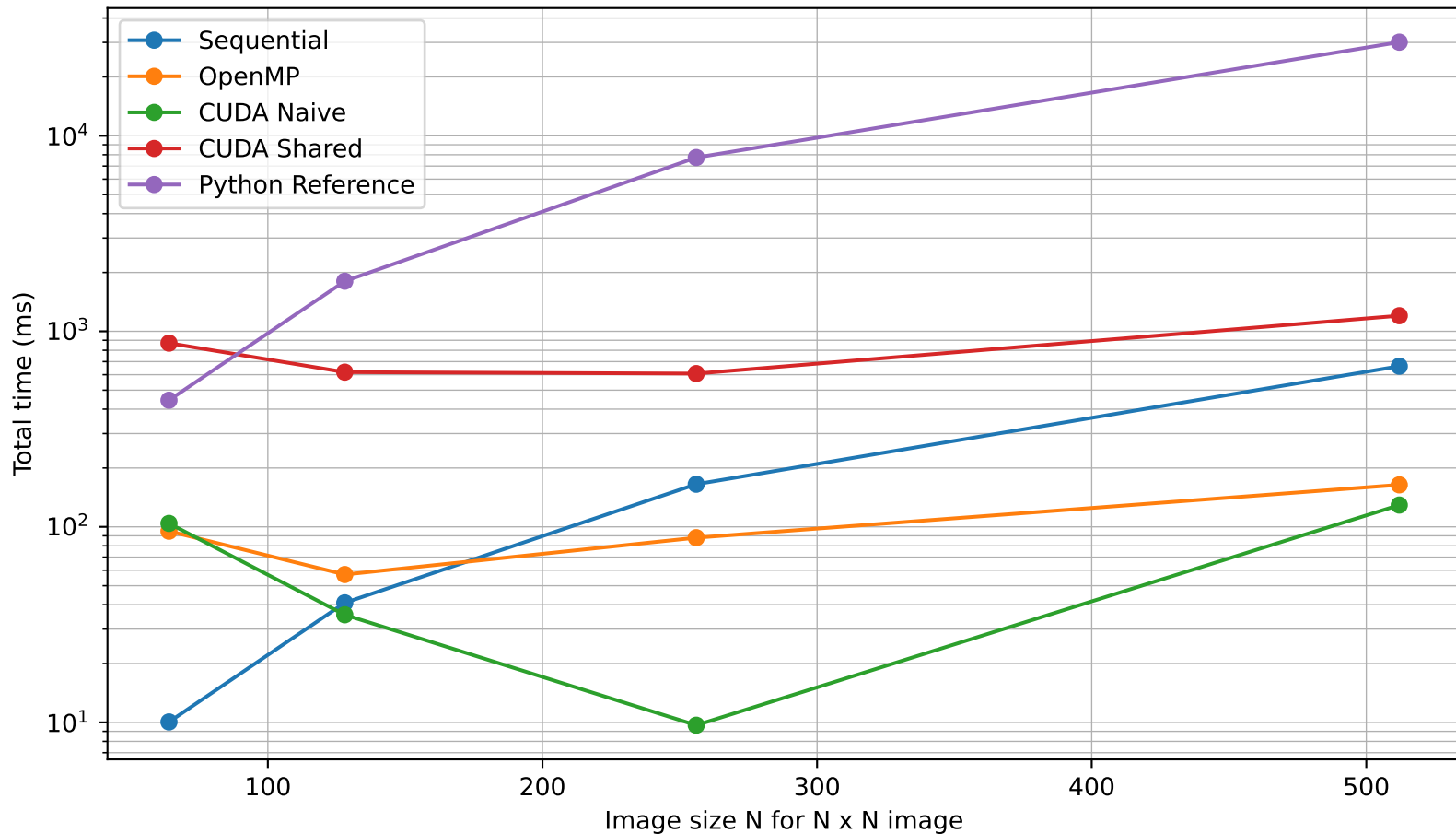
End-to-End Total Time vs Image Size
