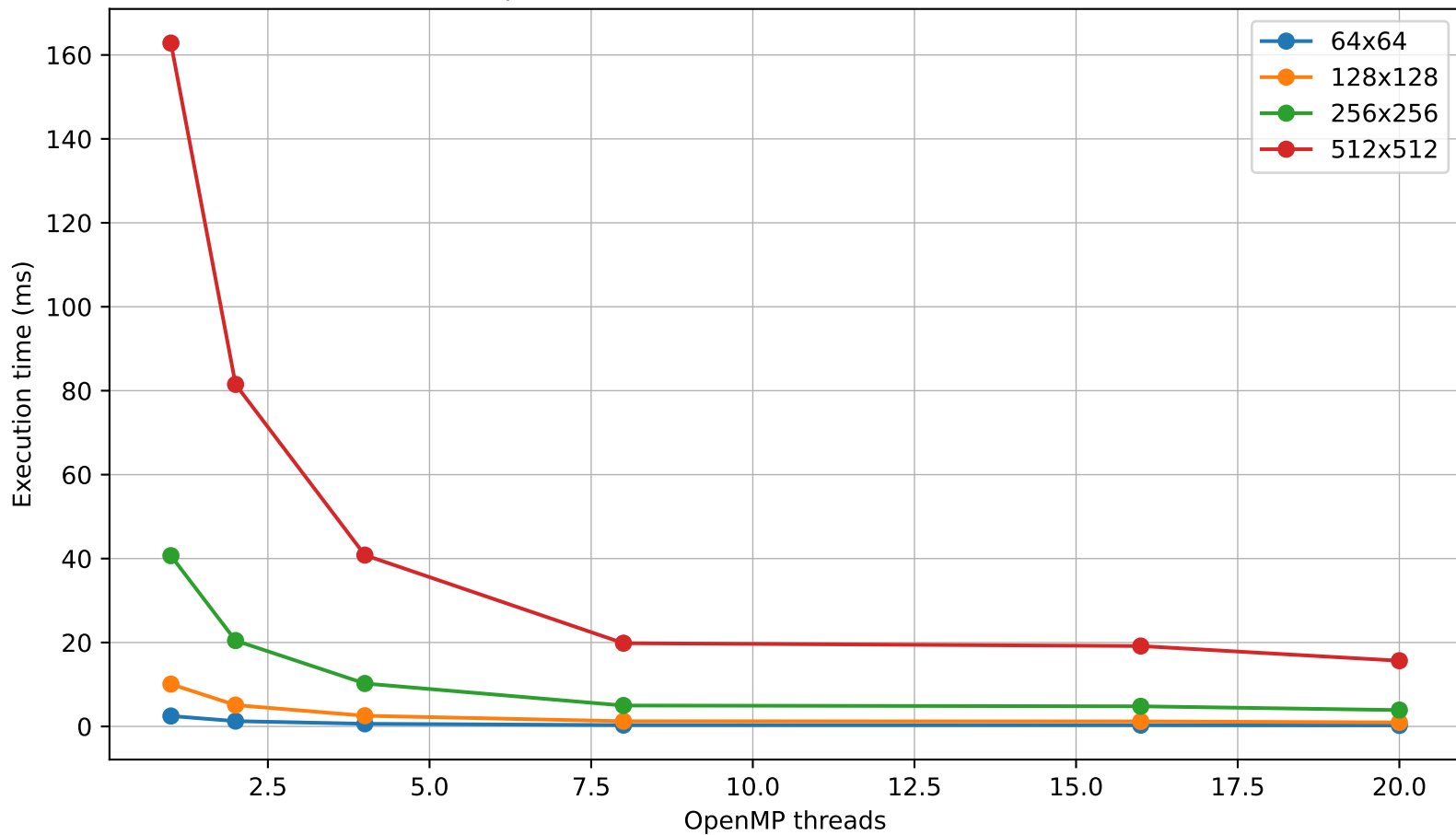
OpenMP Execution Time vs Thread Count
