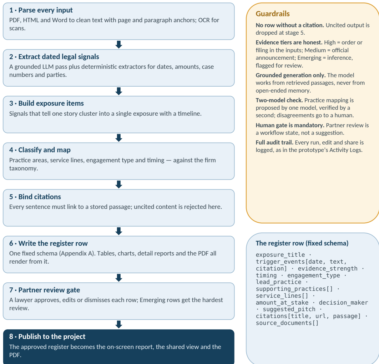
Architecture B — eight stages from raw documents to the approved, published register.
