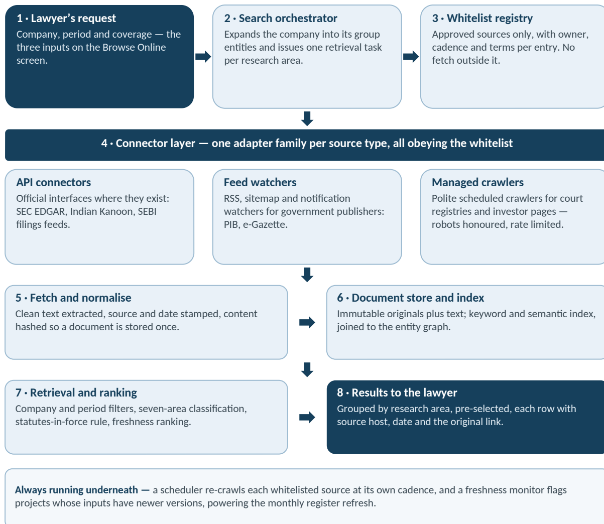
Architecture A — the path from the lawyer's request to the pre-selected result list.
