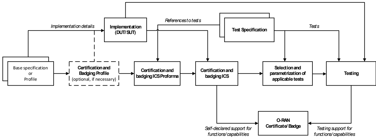
Figure 5.2.1-1: O-RAN Certification and Badging process flow diagram with CB-Profile and CB-ICS proforma
