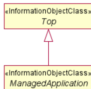
Figure 5.2.2-1: ManagedApplication inheritance
