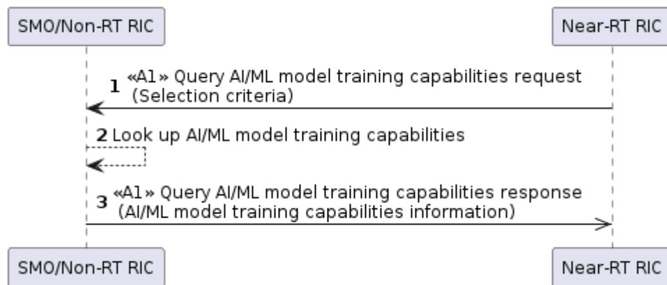
Figure 8.3.3.1-1 Query AI/ML model training capabilities
