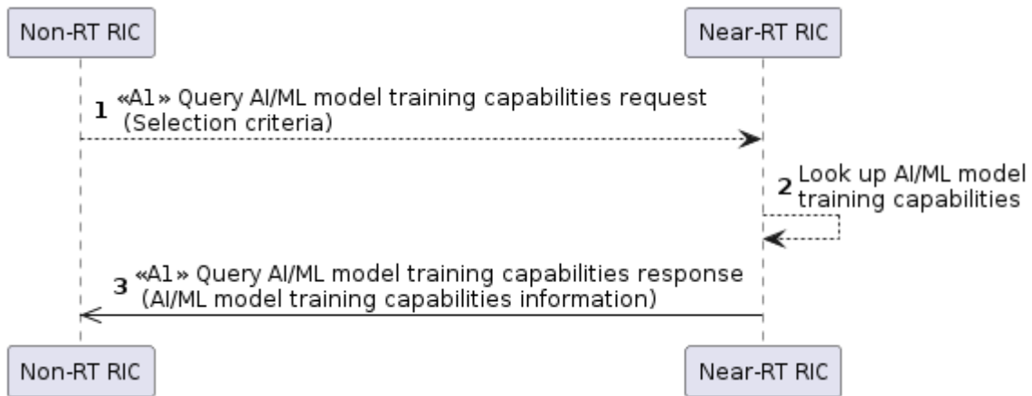
Figure 9.3.3.1-1 Query AI/ML model training capabilities
