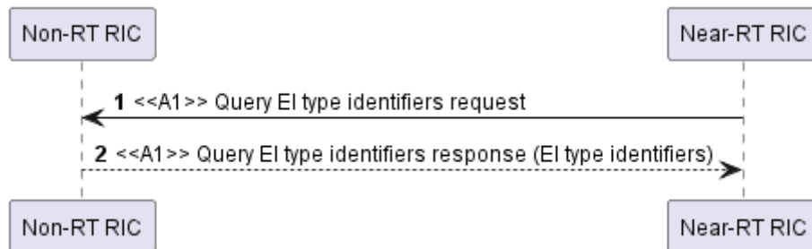
Figure 7.1.3.1-1: Query EI type identifiers
