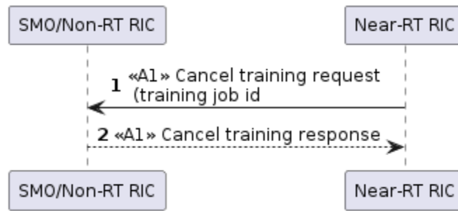
Figure 8.4.3.1-1: Cancel AI/ML model training - Near-RT RIC requests to cancel AI/ML model training
