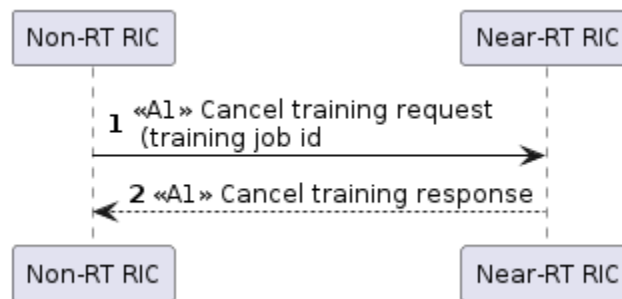
Figure 9.4.3.1-1: Cancel AI/ML model training - Non-RT RIC requests to cancel AI/ML model training
