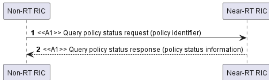
Figure 6.7.3.1-1: Query policy status
