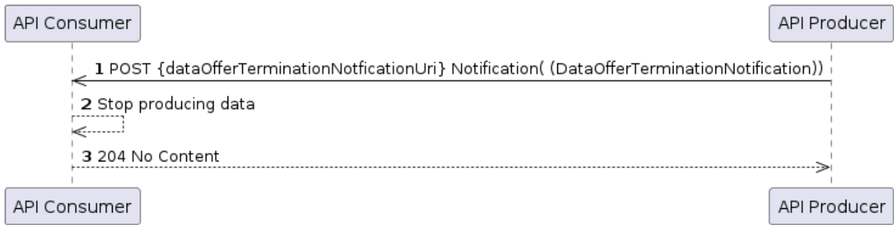
Figure 7.6.4.3.1-1: Notify data offer termination
