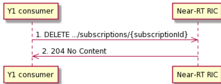
Figure 6.2.3.3.2-1: Y1 consumer unsubscribes from notifications
