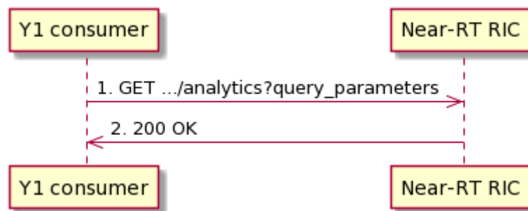
Figure 6.3.3.2.2-1: Y1 consumer query a RAI
