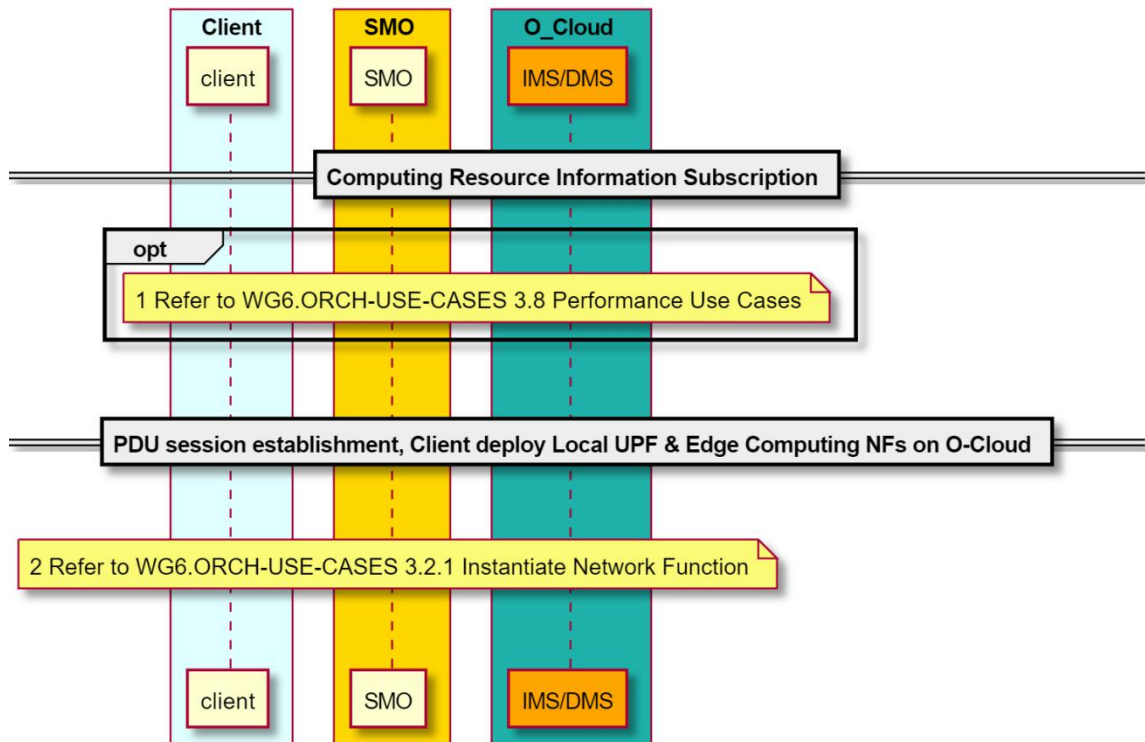
Figure 7.5.3-1: Deploy Edge Computing NFs
