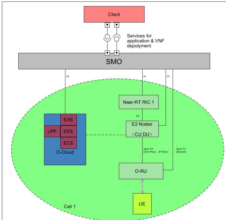
Figure 7.5.2-1: Deploy Edge Computing NFs on O-Cloud
