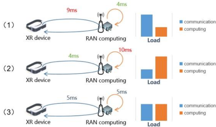
Figure 5.4.2-2: RAN computing nodes with different bandwidth load and computing load
