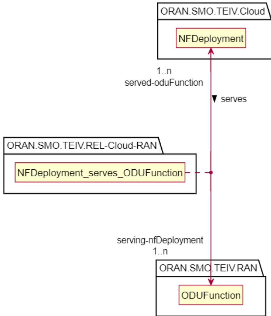
Figure 4.3.3.3.1-3: NFDeployment and ODUFFunction relationship model
