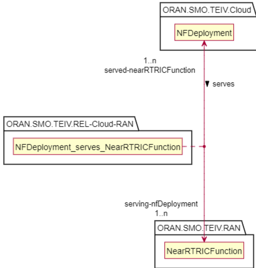
Figure 4.3.3.3.1-6: NFDeployment and NearRTRICFunction relationship model
