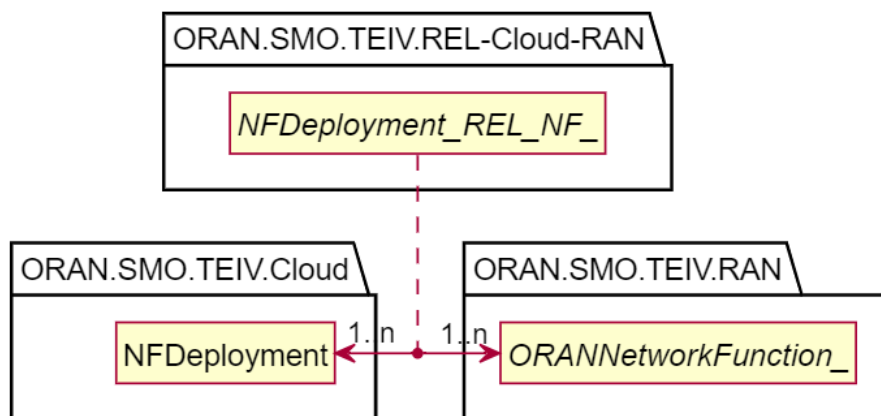
Figure 4.3.3.3.1-1: SMO TE&IV Cloud-RAN relationship model
