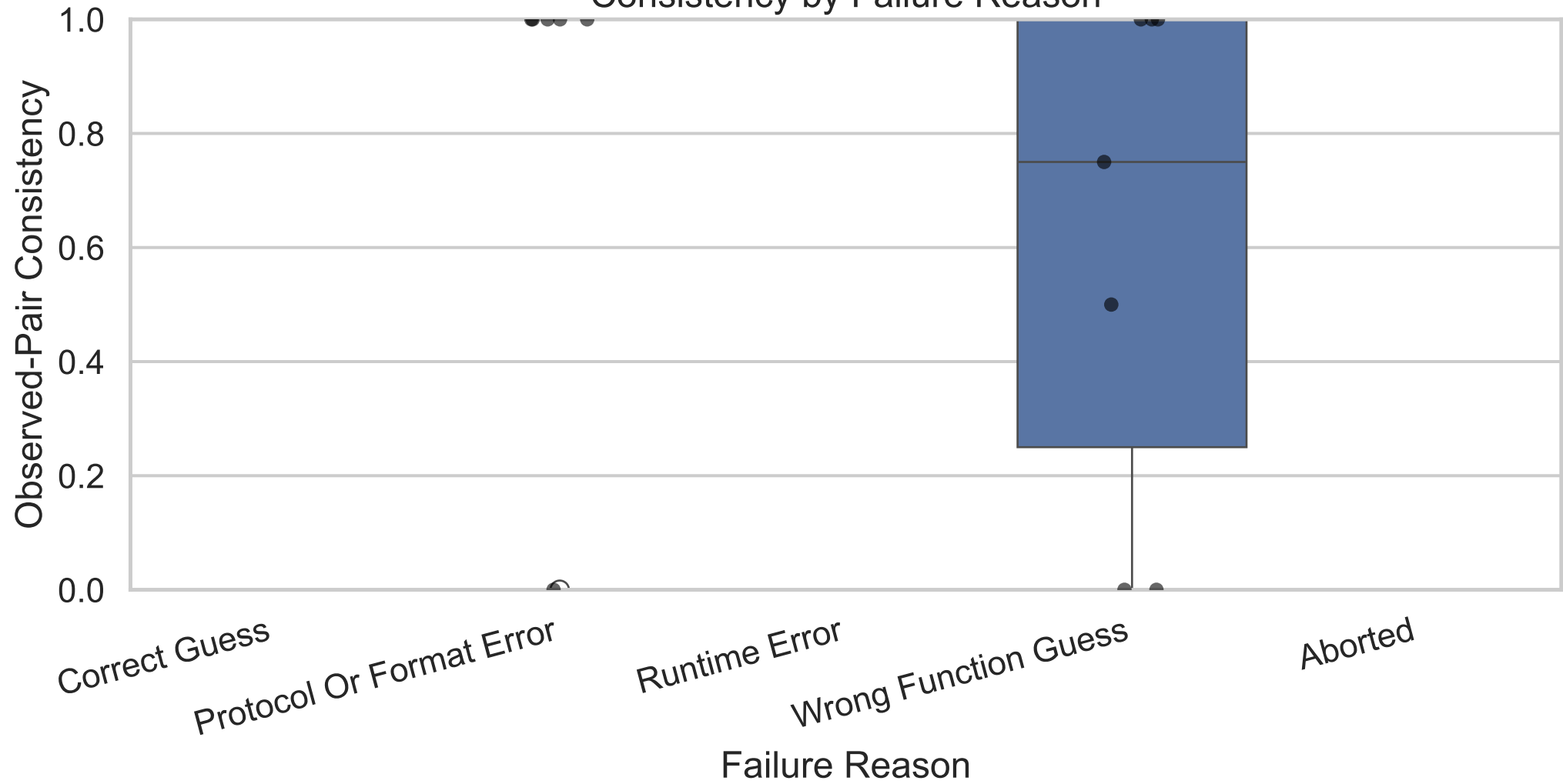
Consistency by Failure Reason
