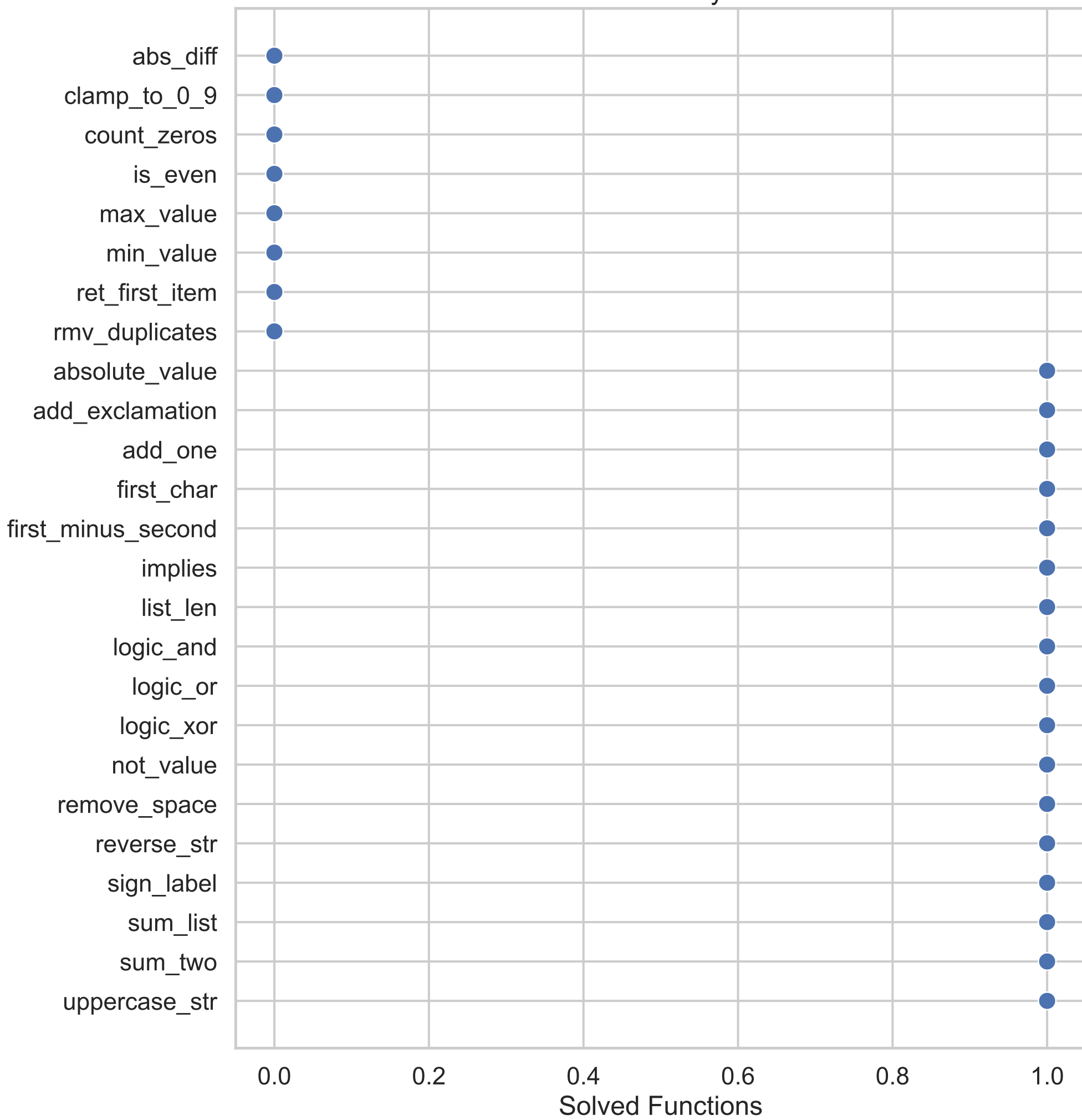
Correct Guesses by Function
