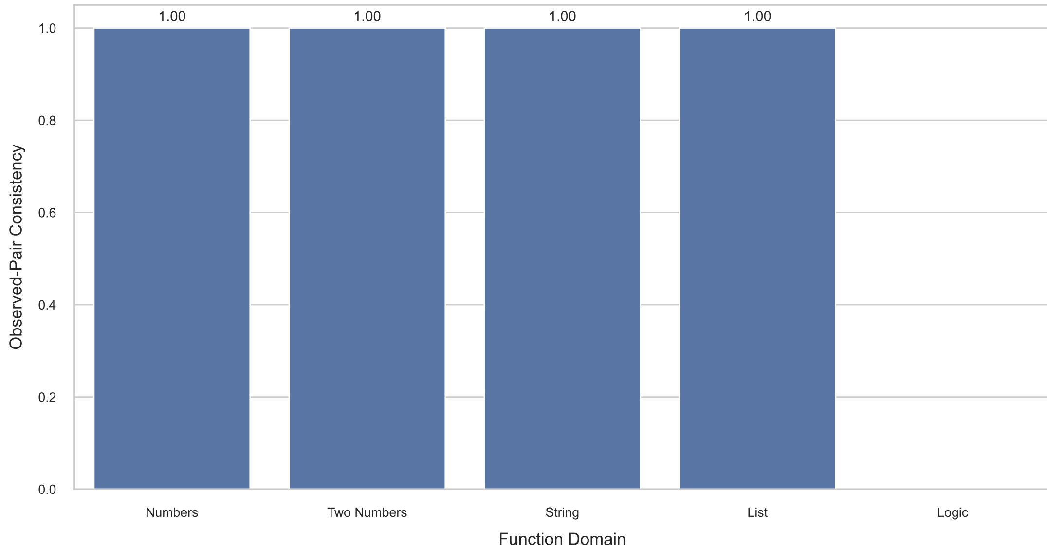
Observed-Pair Consistency on Failed Episodes by Domain
