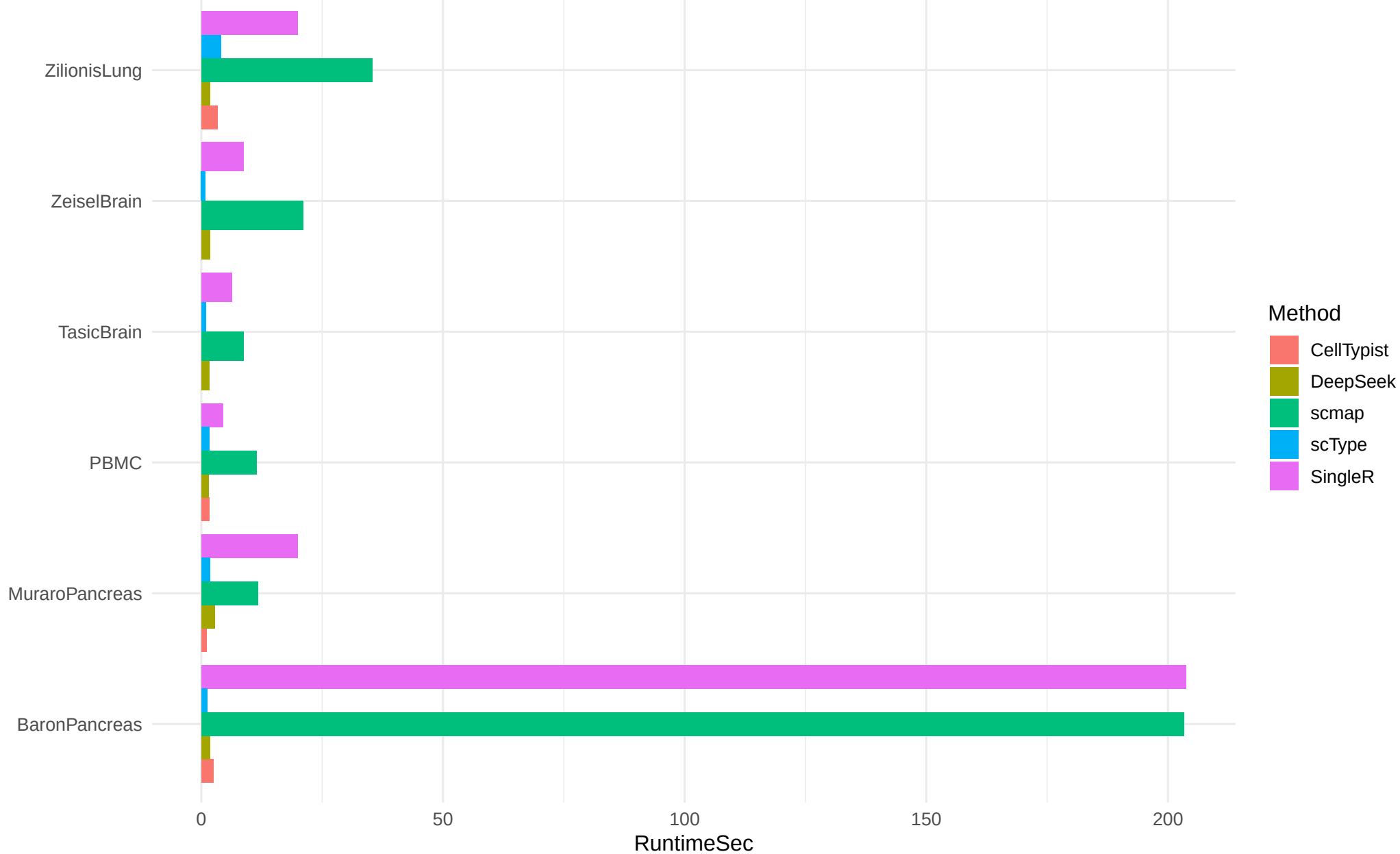
DeepSeekCell benchmark: RuntimeSec
