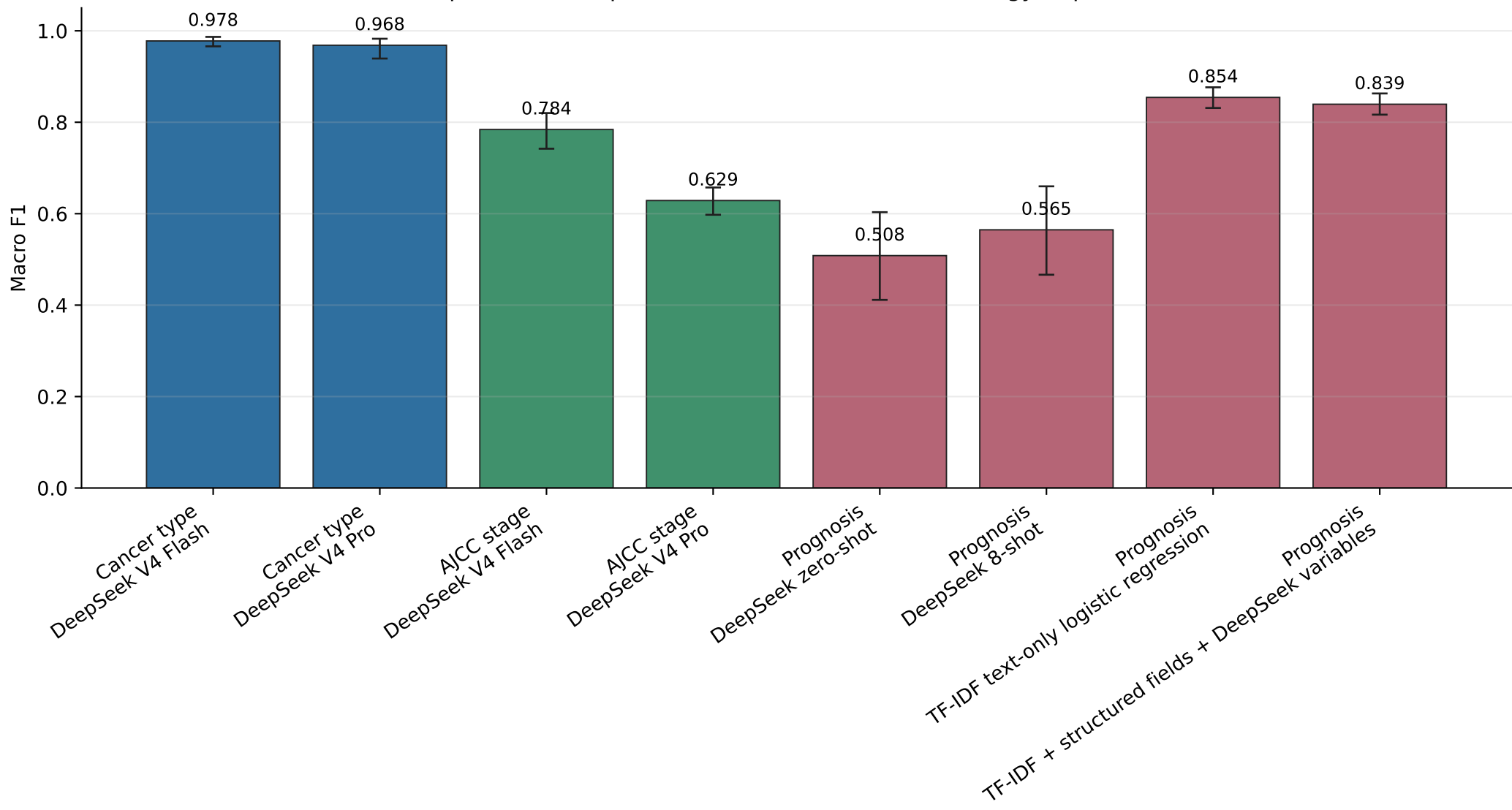
DeepSeek and Supervised Baselines Across Pathology Report Tasks
