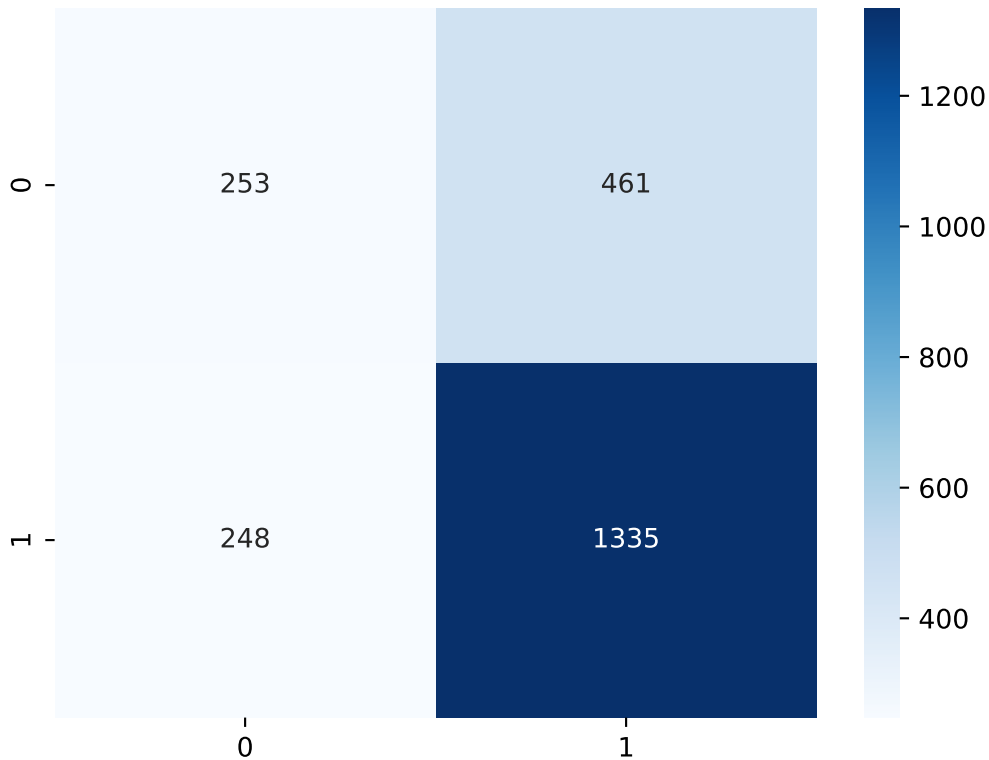
Confusion Matrix - distilbert
