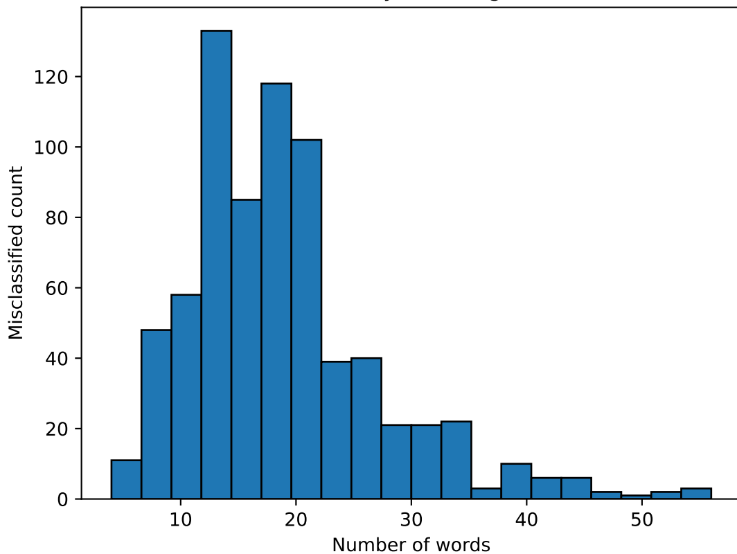
Misclassification by text length - Baseline
