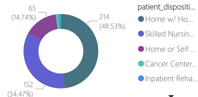
Total Discharges by patient_disposition
