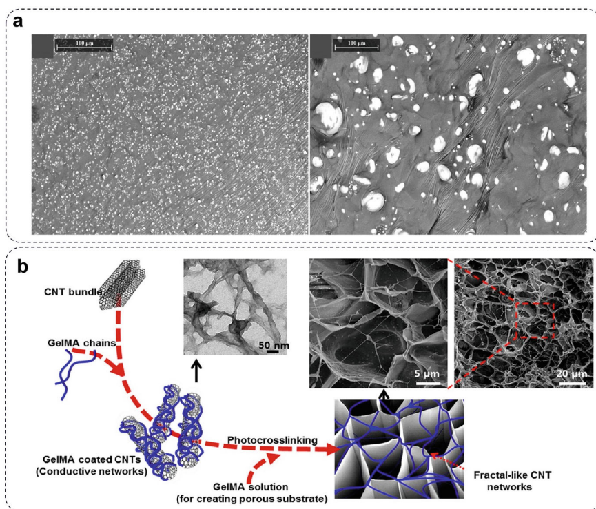
Fig. 3.2 a FESEM images showing the microstructural arrangement of soft and hard magnetic magnetorheological elastomers prior to magnetic actuation. Reproduced from [9] with permission. b Microstructure of fractal-like carbon nanotube (CNT) networks embedded in GelMA hydrogel. Nanofibrous networks are visible both across and within the porous structure. Reproduced from [10] with permission
