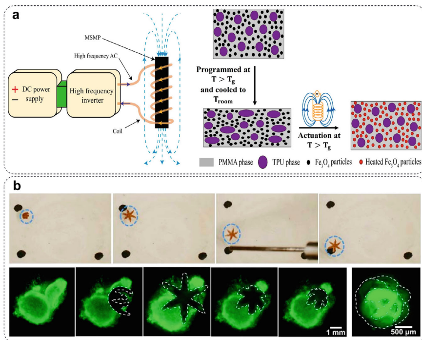
Fig. 3.8 a Induction heating setup used for heating up PMMA/TPU/Fe 3 O 4 Shape memory polymer composites. Adapted from [90] under the CC BY-NC 4.0 license. Shape changing mechanism is shown. b Applications of soft thermo-responsive self-folding microgrippers for precise magnetic guidance, cell capture, and excision from a live fibroblast clump. Reproduced from [99] with permission. Copyright © 2015 American Chemical Society
