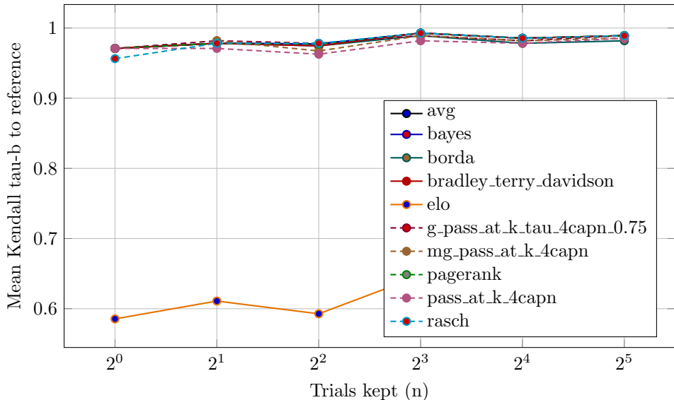
Ranking Stability vs Trials
