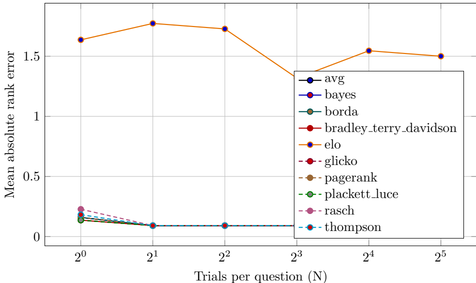
Synthetic Rank Recovery: Mean Absolute Rank Error
