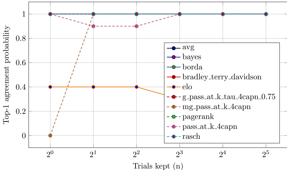
Top-1 Stability vs Trials
