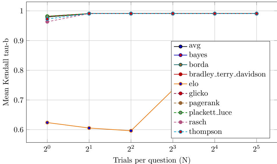
Synthetic Rank Recovery: Kendall tau-b
