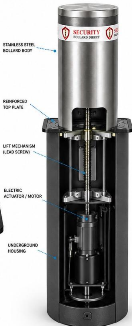
AUTOMATIC / CUTAWAY VIEW
