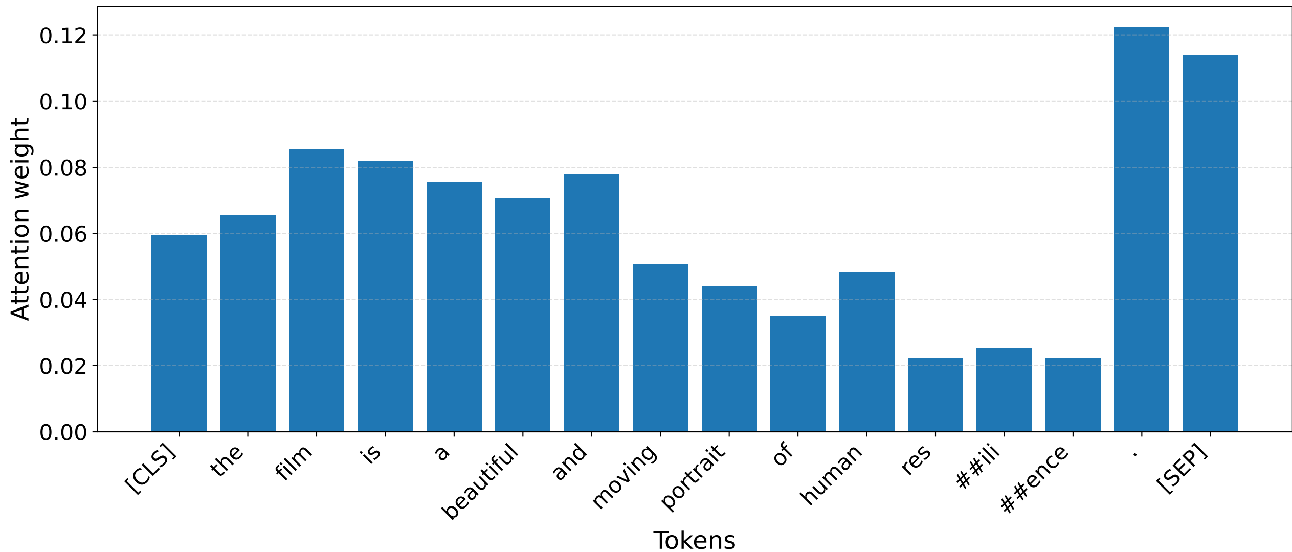
S1 [POS] — Vanilla attention CLS row
