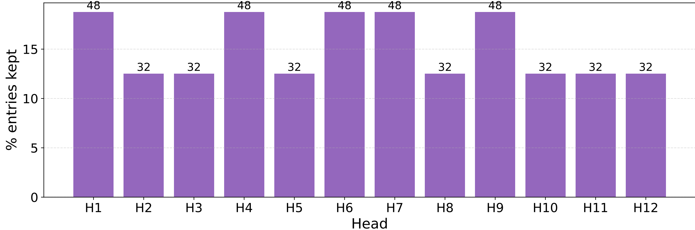
S1 Step 2 — Mask sparsity per head (K=0.3)
