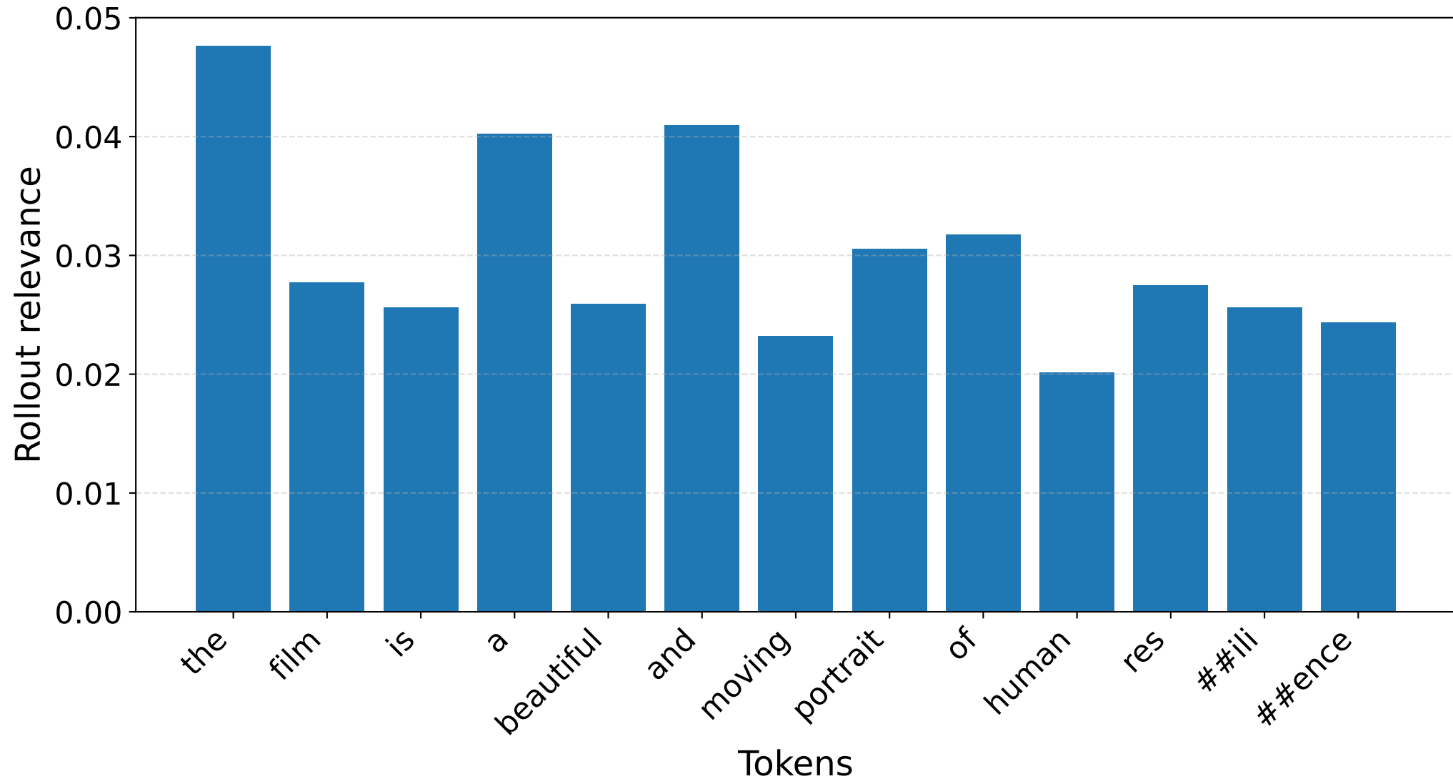
S1 [POS] — Standard rollout CLS row (filtered tokens)
