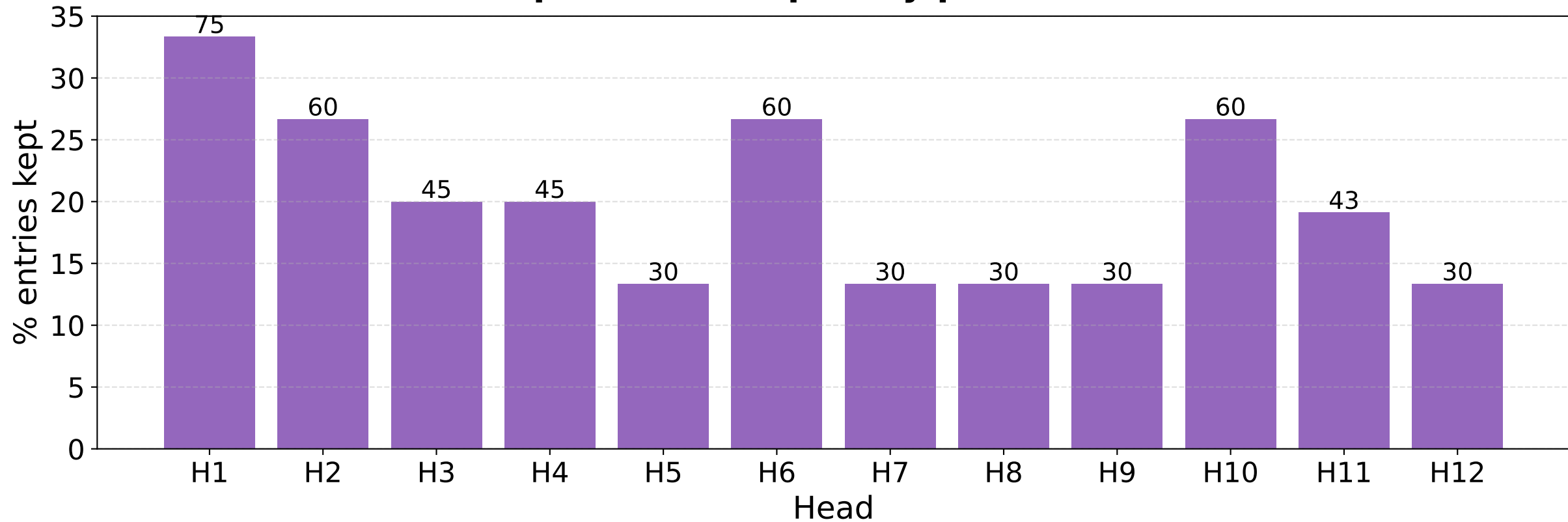
S10 Step 2 — Mask sparsity per head (K=0.0)
