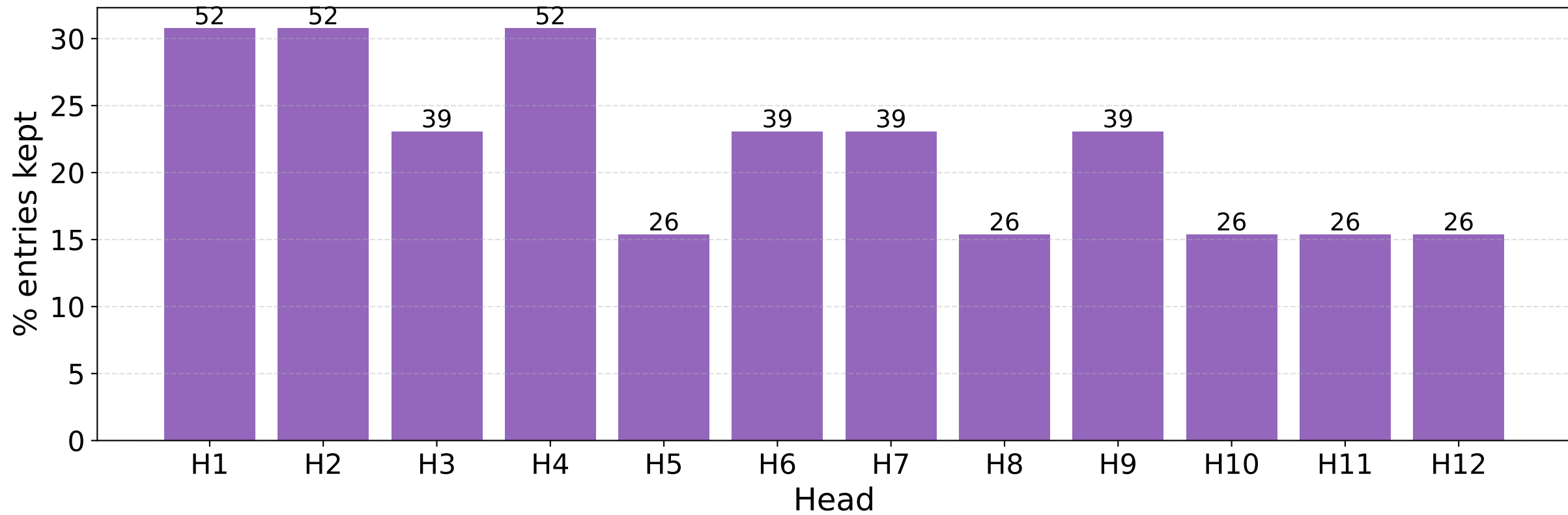
S2 Step 2 — Mask sparsity per head (K=0.0)
