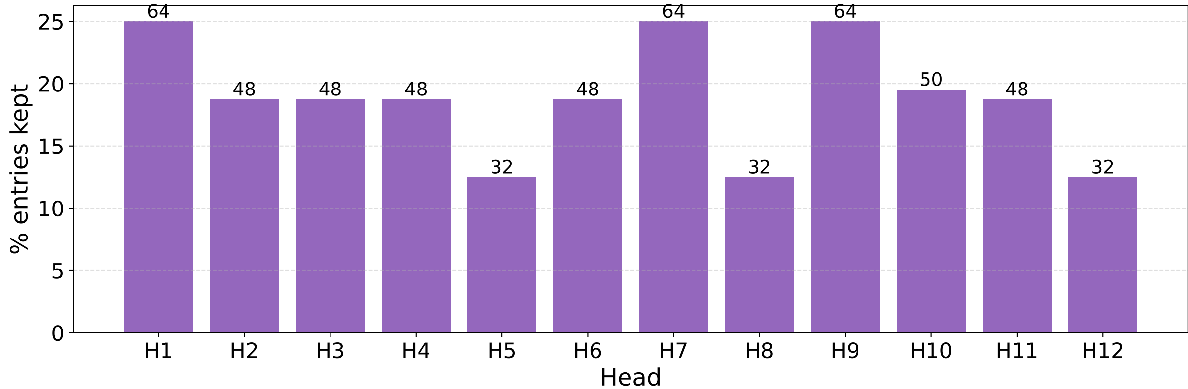
S3 Step 2 — Mask sparsity per head (K=0.0)
