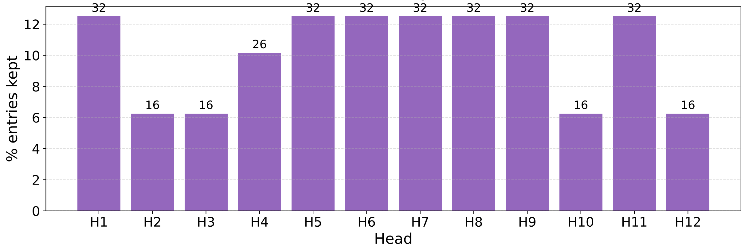
S3 Step 2 — Mask sparsity per head (K=1.0)
