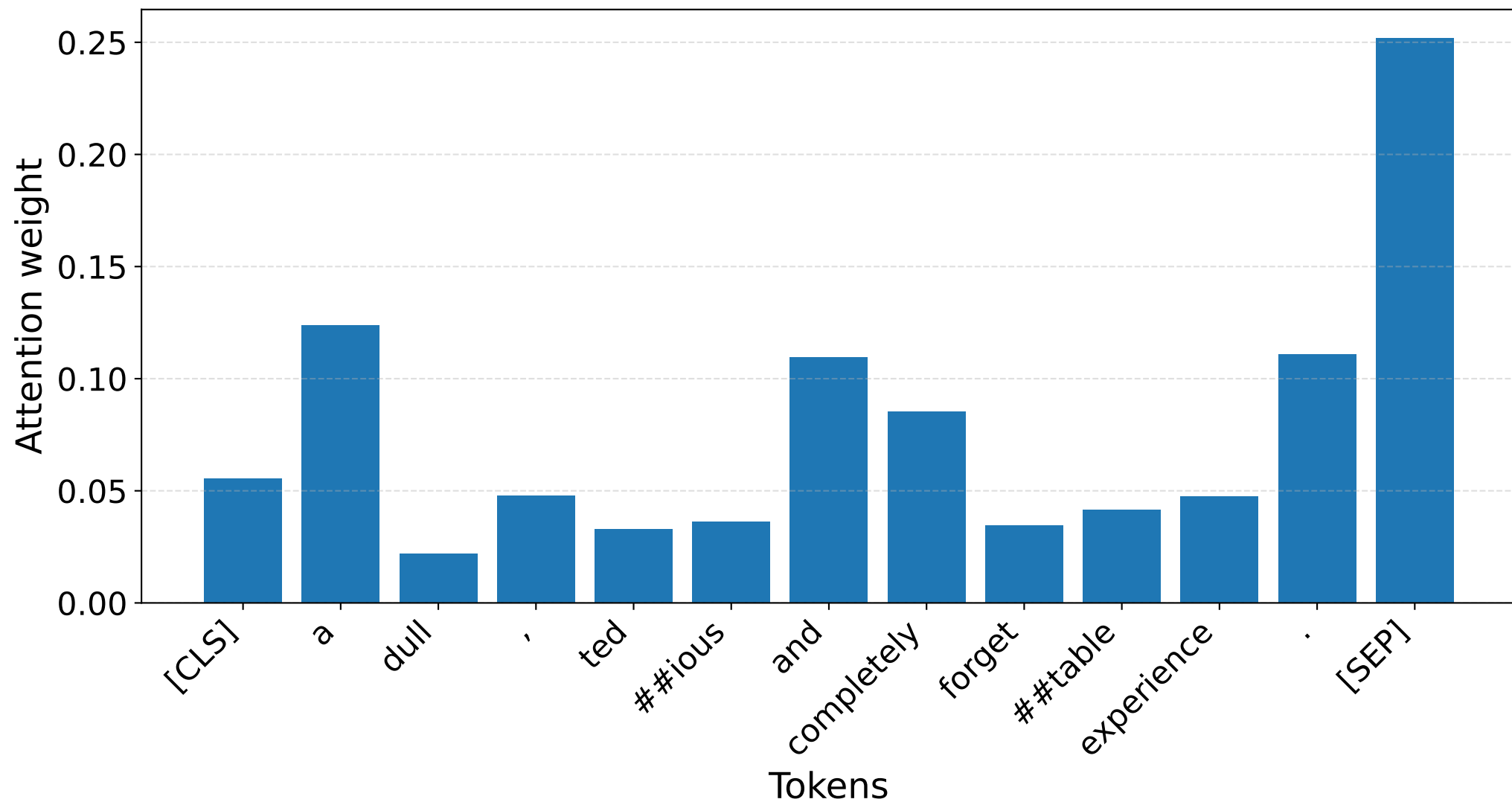
S4 [NEG] — Vanilla attention CLS row (Layer 1, Head 1)
