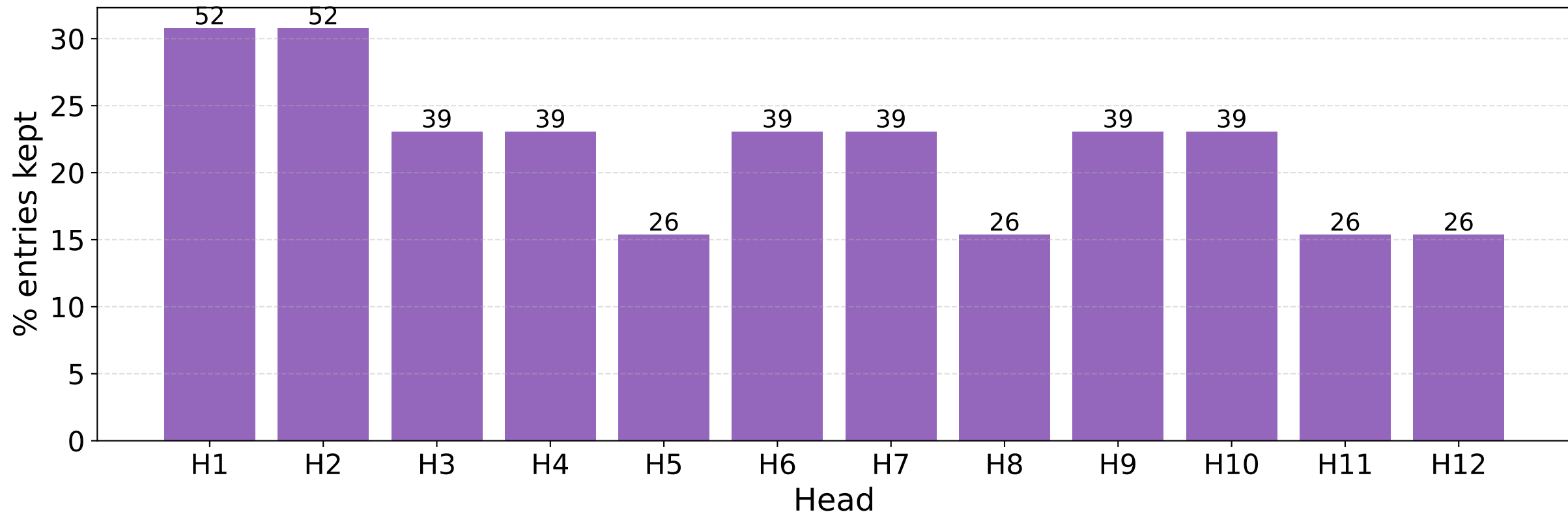
S4 Step 2 — Mask sparsity per head (K=0.0)
