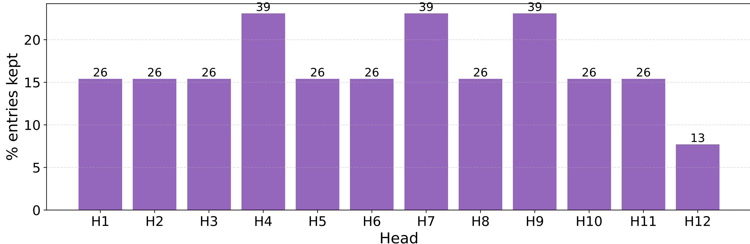
S4 Step 2 — Mask sparsity per head (K=0.5)
