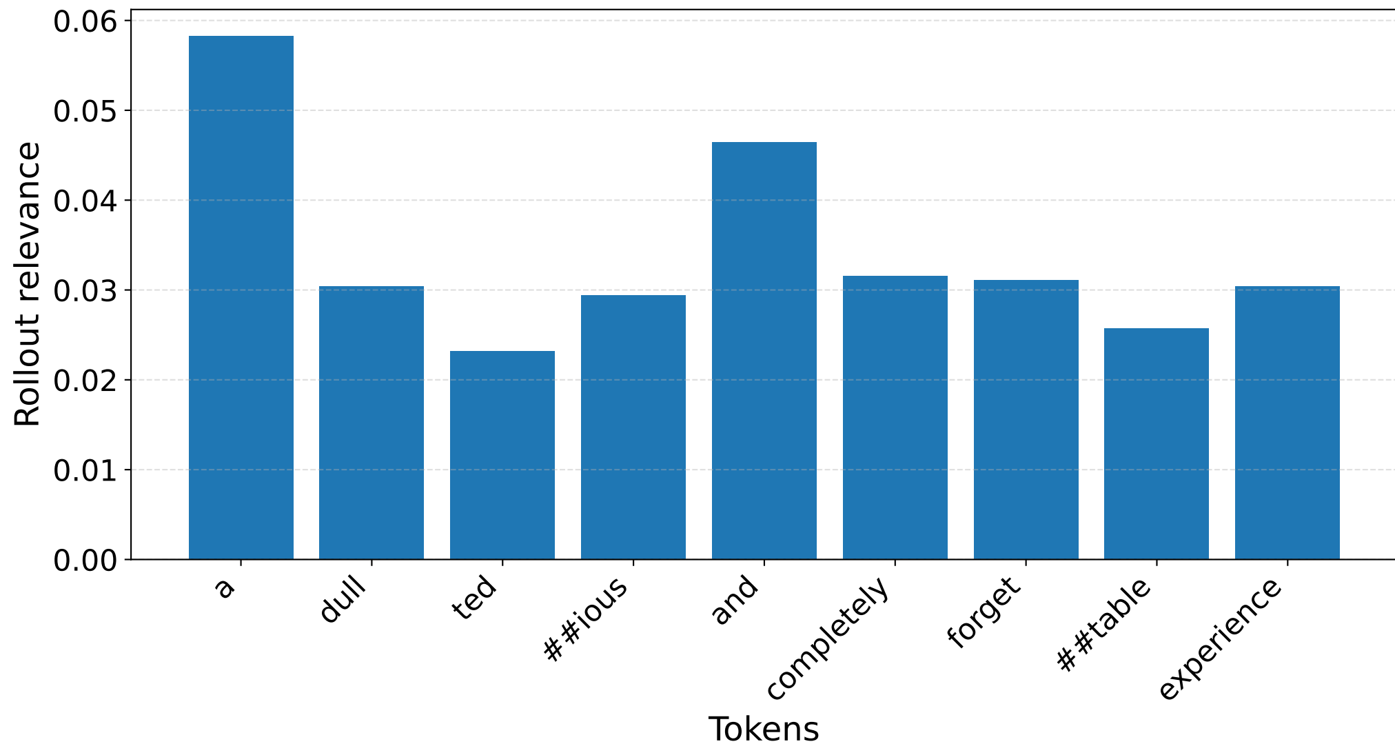
S4 [NEG] — Standard rollout CLS row (filtered tokens)
