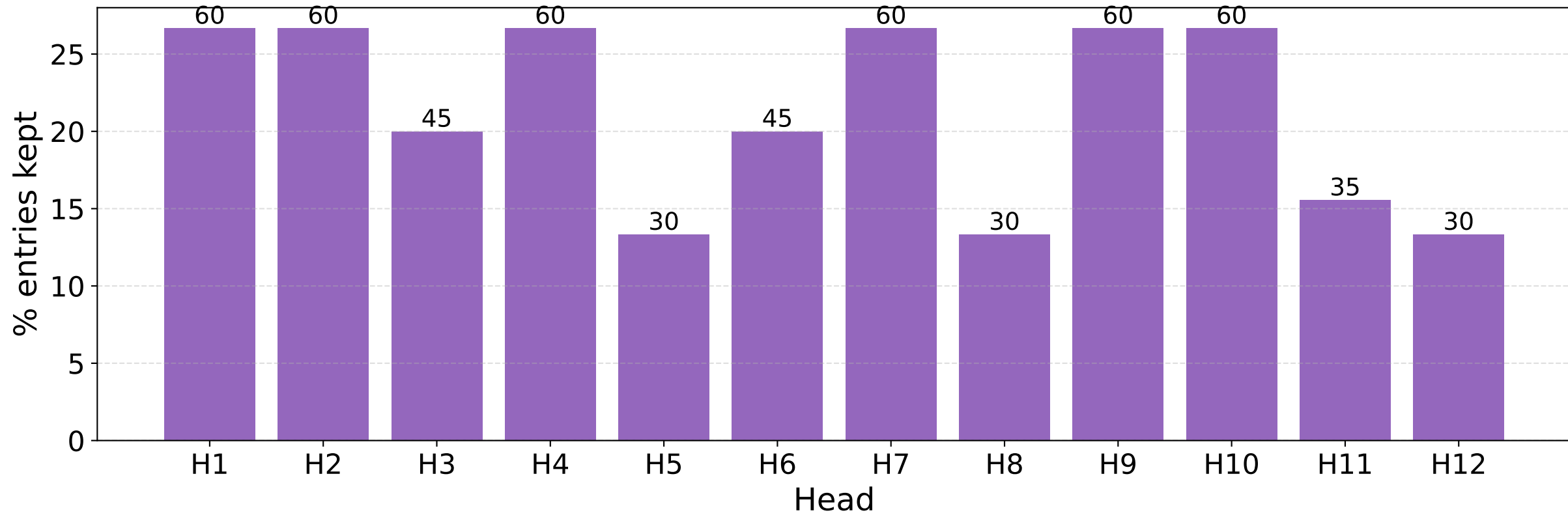
S5 Step 2 — Mask sparsity per head (K=0.0)
