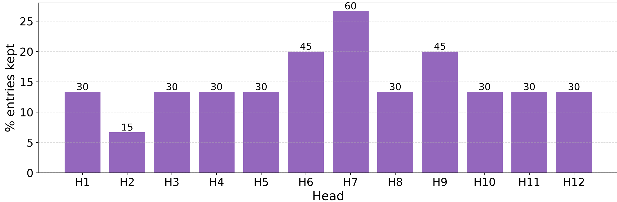
S5 Step 2 — Mask sparsity per head (K=0.5)
