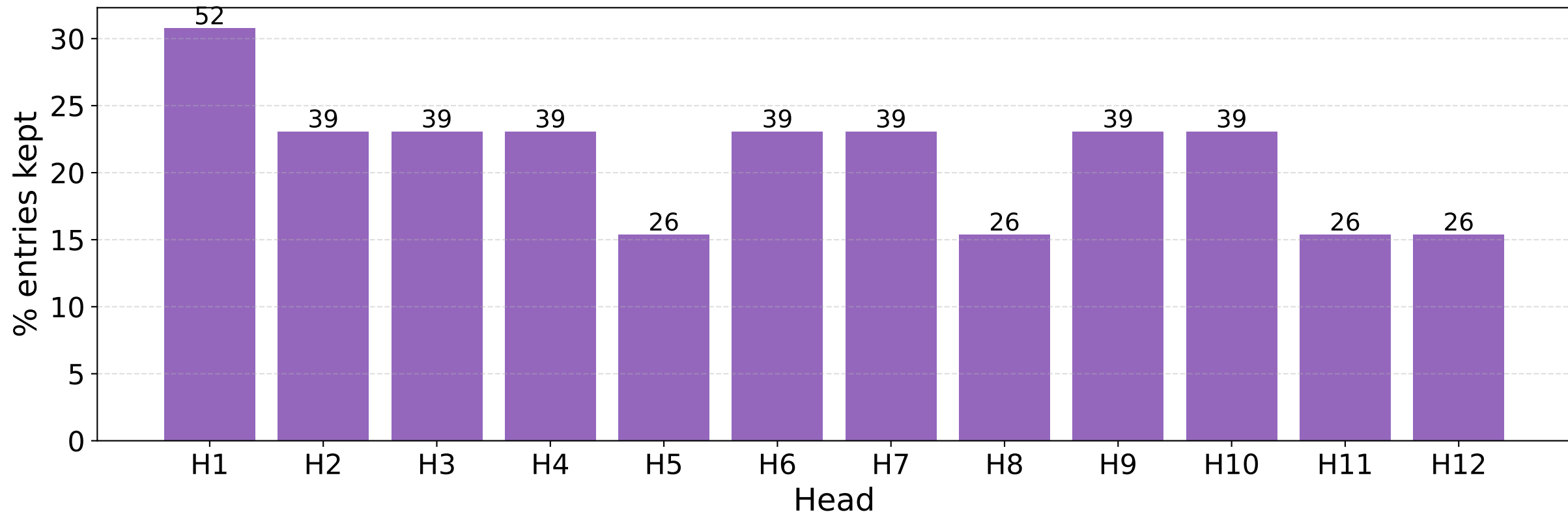
S6 Step 2 — Mask sparsity per head (K=0.0)
