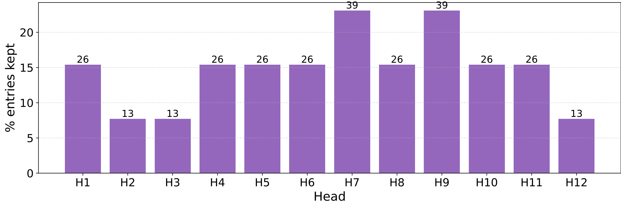
S6 Step 2 — Mask sparsity per head (K=0.5)
